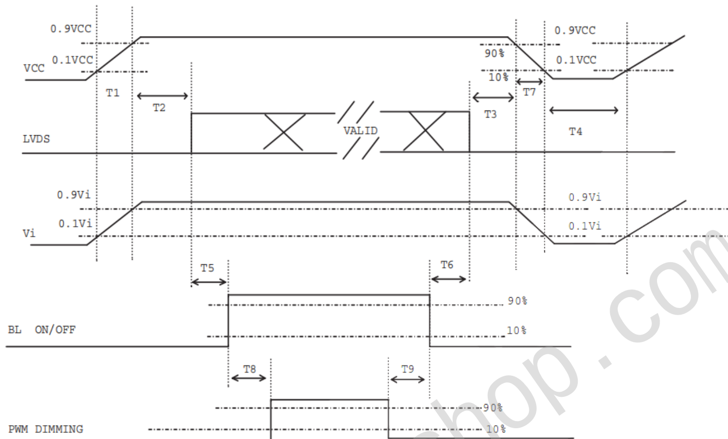
Power ON/OFF sequence
