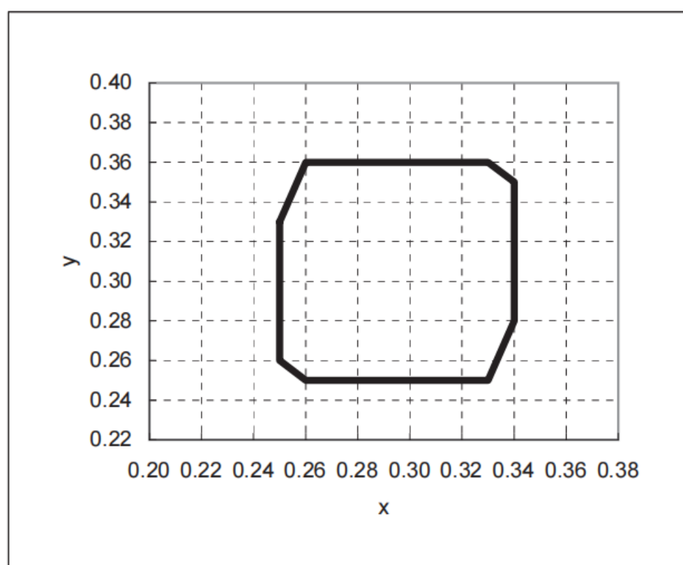
White Chromaticity Range
